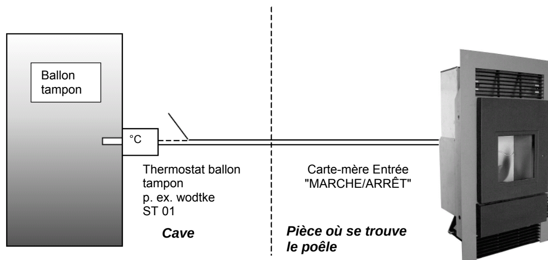
Ex. 1.3.0: Raccordement via le thermostat ballon tampon (sans potentiel)
